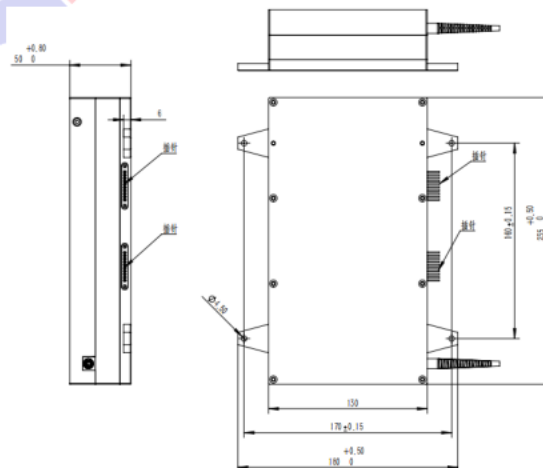
PIC 2-2 50W Green Light Dimensions
