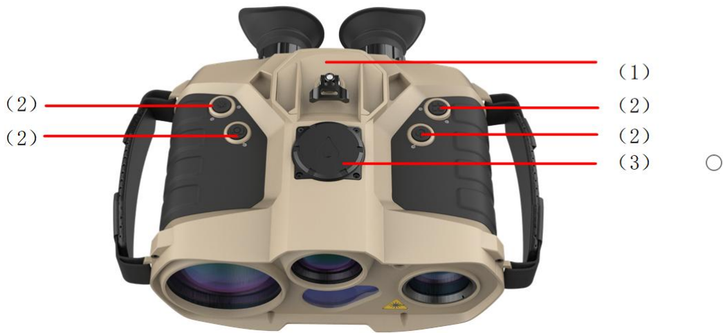
Figure 2 Top of binoculars
