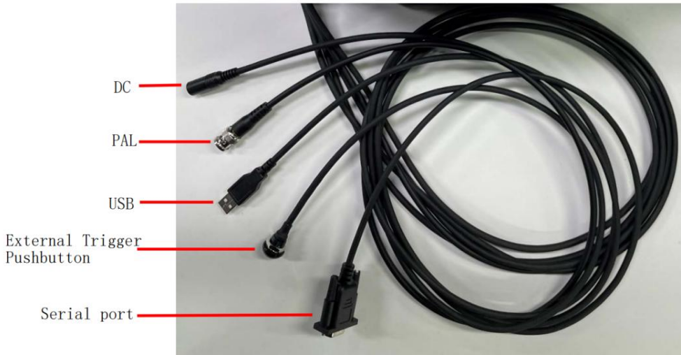
Figure 6 Aerial Plug Cables
